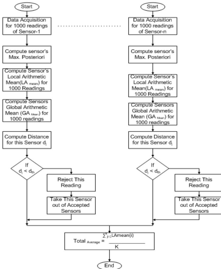
Figure 4. Flow chart shows how sensor similarity is performed.
