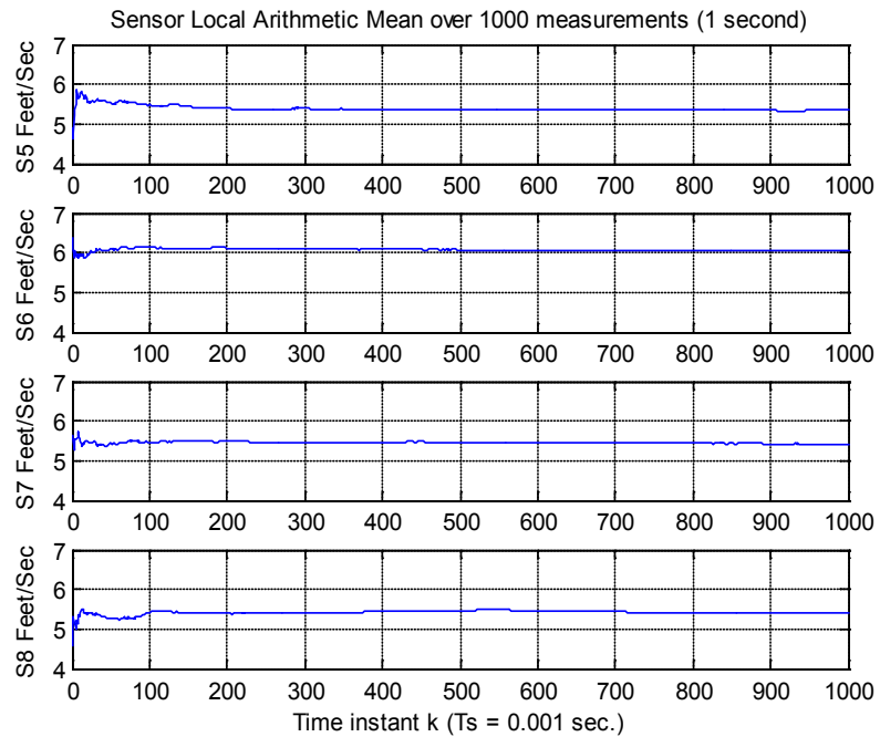
Figure 10. Local arithmetic mean (LAmean) for the four sensors on the Y-axis over 1 second time span
